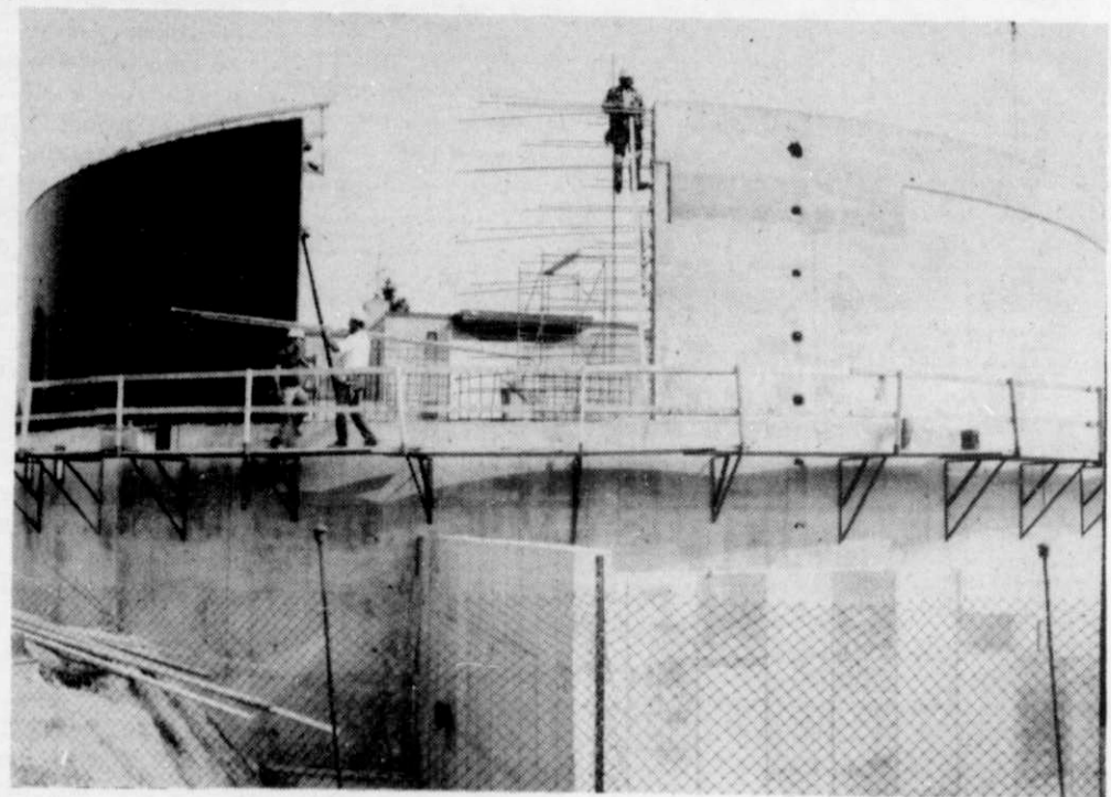
Construction continues on the new bio-solid storage tank for the Kewaskum Wastewater Treatment Plant for the village. With a capacity to hold 1.1 million gallons of sludge, the tank should be completed in October. Pictured above are two phases of construction by C.D. Smith Construction of Fond du Lac. The top photo shows the crew finishing the foundation or floor, and the bottom photo taken this week, features the erection of the concrete walls for the pump room.
