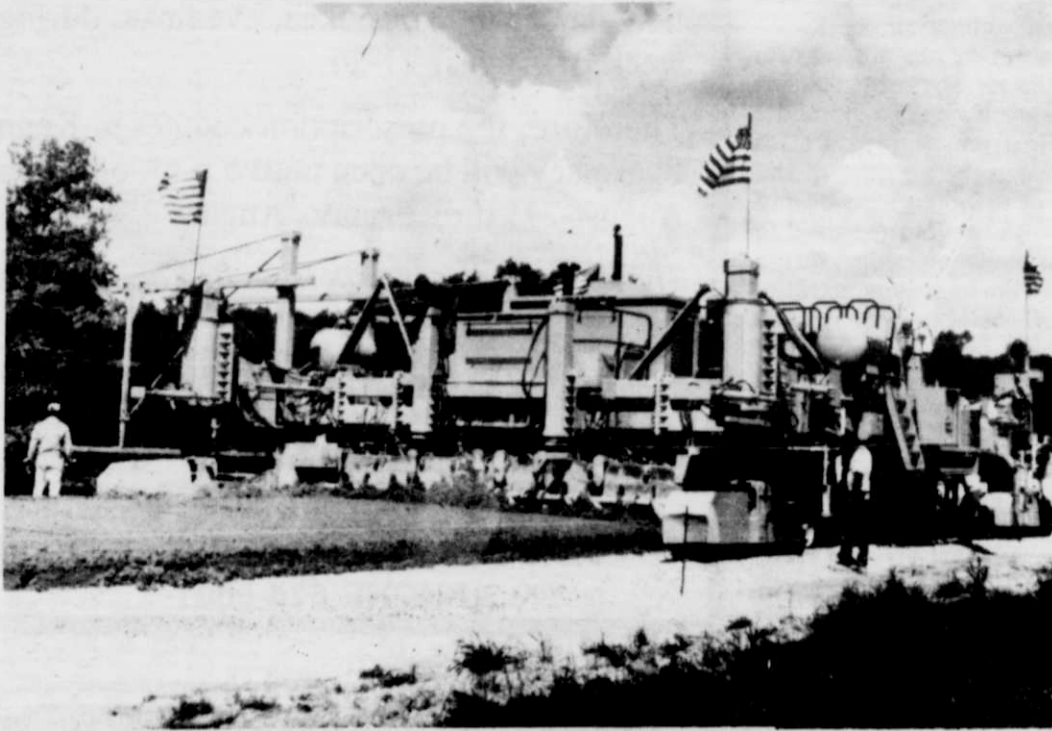
The state-of-the-art paver manufactured by Gomaco, Inc., of Iowa, is computer-controlled, laying approximately one mile of two-lane wide concrete roadbed per day on the final two lanes of the Highway 45 bypass.
