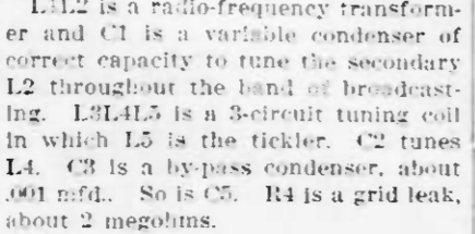
Using Unit Same as Radio Frequency Transformer in Neurodyne Set.
