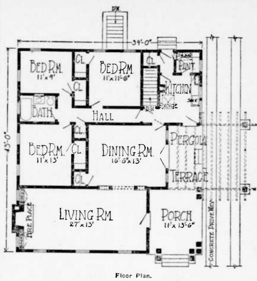
Floor Plan.
