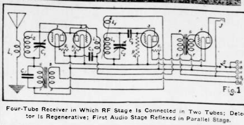
Four-Tube Receiver in Which RF Stage Is Connected in Two Tubes; Detector Is Regenerative; First Audio Stage Reflexed in Parallel Stages.
