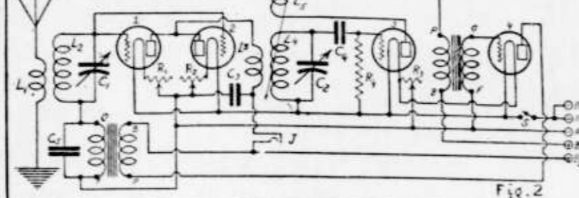
Diagram Showing Same Circuit as That in Fig. 1, Except That the Second Audio Stage is the Reflexed One, Instead of the First.
