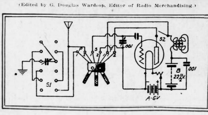
Showing Circuit Diagram of the Conventional Three-Coil Honeycomb, but With Slight Modification.
